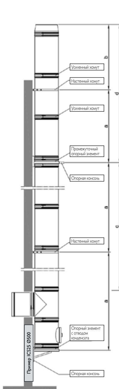
ICS25 Ø350-Ø700
